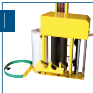
Power Pre-Stretch Carriage
